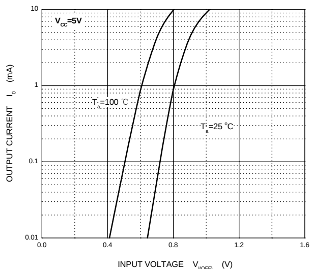
OFF Characteristics
